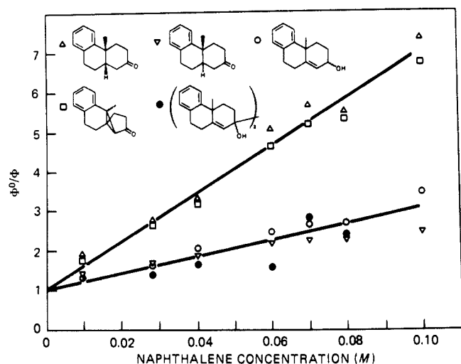
Figure 1. Stern-Volmer plots for quenching the photochemistry of 4-methyl-4,4a,9,10-tetrahydro-2(3H)-phenanthrone ( 1 ) by naphthalene in isopropyl alcohol.
