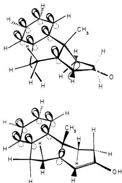
Figure 4. (a, top) Model of the relaxed {}^3\pi,\pi^* excited state of phenanthrone 1 . (b, bottom) Model of the hydroxyallyl radical derived from the {}^3\pi,\pi^* excited state of phenanthrone 1 by H-atom abstraction from isopropyl alcohol.
